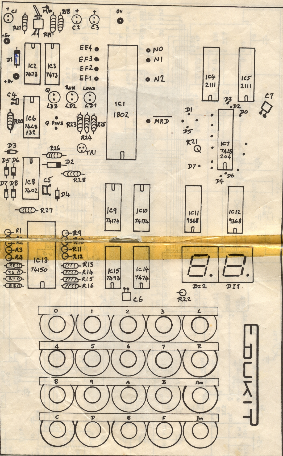
COMPONENT OVERLAY DIAGRAM
